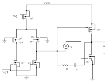
Figure 3. the circuit with body-driven input
