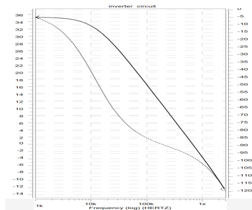
Figure 4. Frequency response of the circuit in Figure 3
