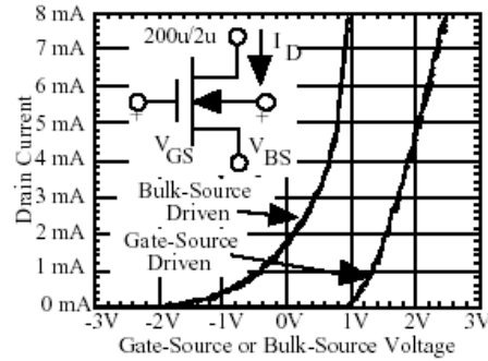
Figure 1. the drain current with respect to body-source and gate - source voltage
