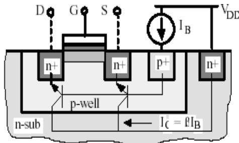
Figure 2. internal structure of an NMOS
