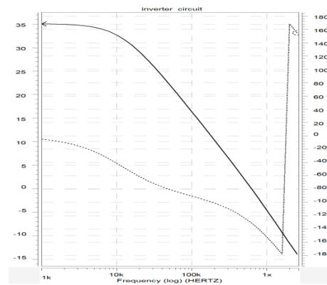
Figure 6. Frequency response of the circuit in Figure 5
