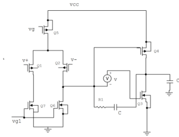
Figure 5. the proposed circuit which all devices are biased in sub-threshold region
