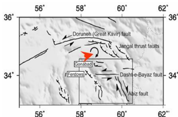
Figure 8. Clockwise rotation of the Lut block and left-lateral activity of the Drouneh Fault at its northern margin, certainly had direct role in transcurent faulting inward of the northern Lut with similar behavior dependent to this system. Schematic map from Walker, (2004)
