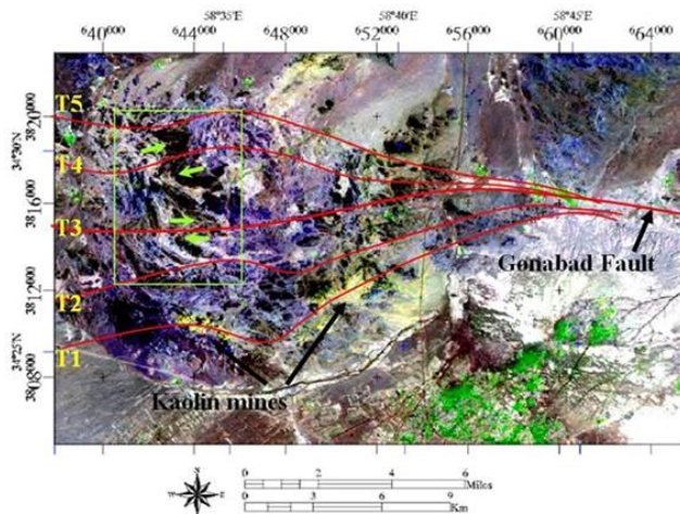
Figure 7. Horsetail structure can be seen on Landsat TM image-map in the right half of defined window overlapped to end of Gonabad Fault. Conjunction of quintuplicate branches with Gonabad Fault was certified at the best style. By readily ascent of hydrothermal fluids through the T1, it is considered as the main structure that has controlled location of faulted argillic alterations and kaolin mines. T3 at the middle of the system which has longer displacement (approximately 3 km), is original branch that directly attached to Gonabad Fault. Large right-lateral displacement during third episode marked in the green quadrangle. Dynamics of these assemblages have been interpreted in sequences of arc evolution model as follow
